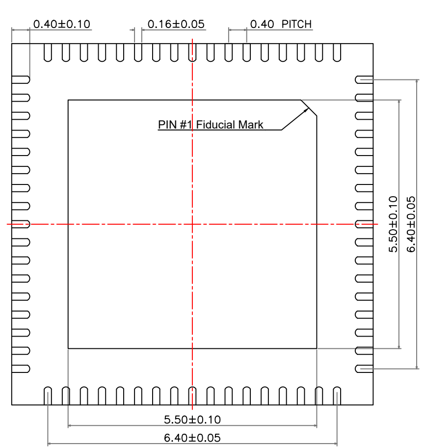
BOTTOM VIEW
